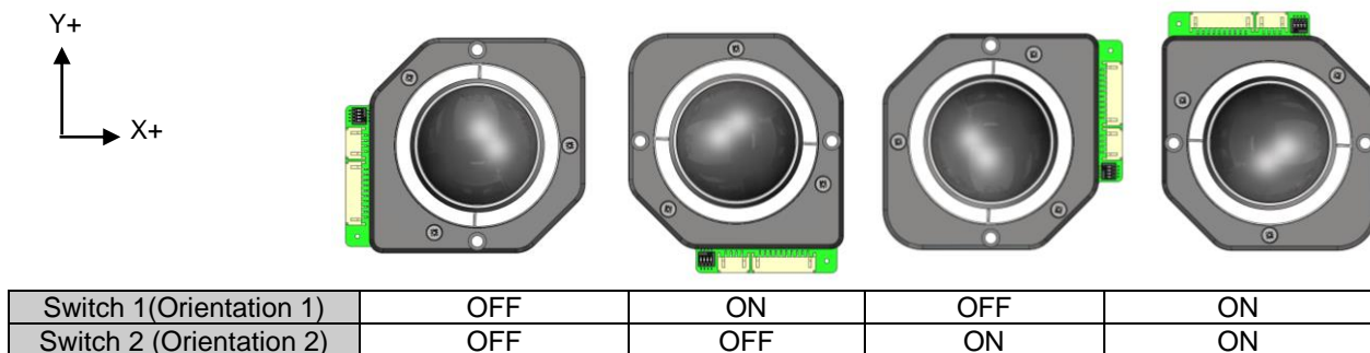
Figure 1 – Mounting Orientations
